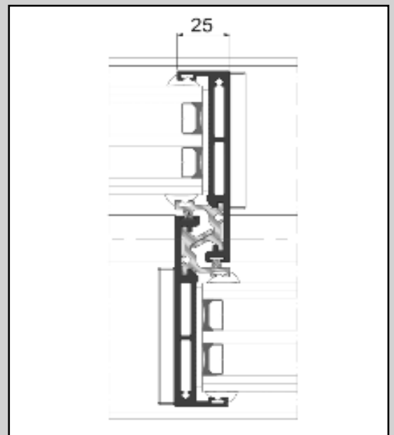
Meeting Stile/ Interlock Section
