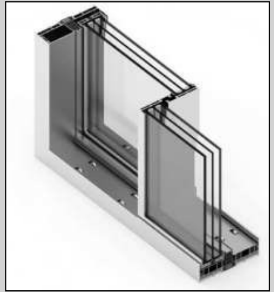
2 Track Jamb Section
